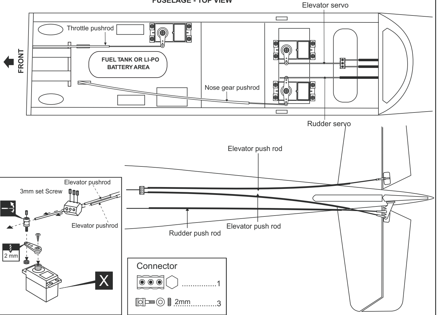
FUSELAGE - TOP VIEW
