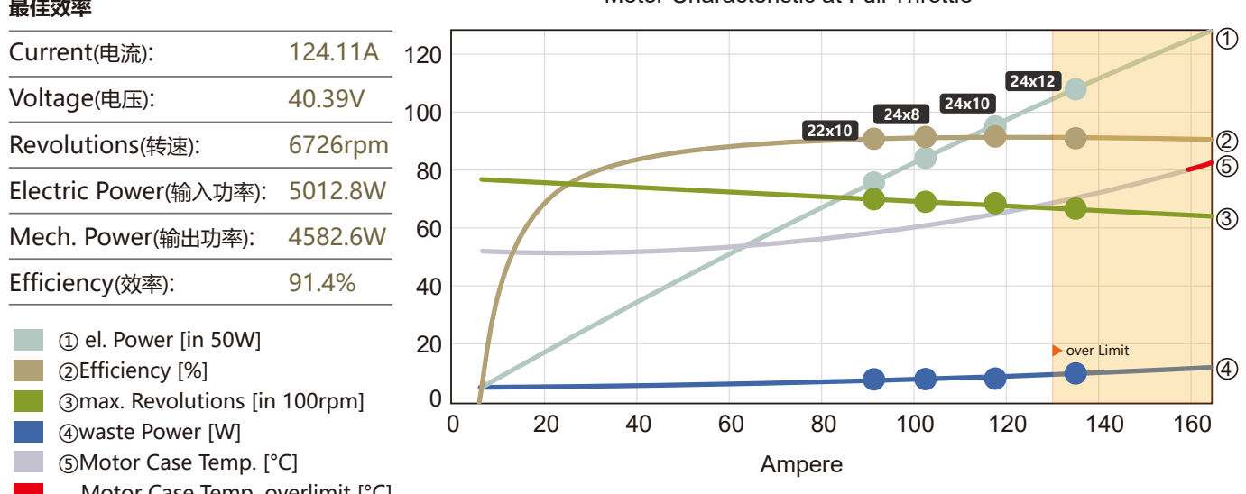
Motor Characteristic at Full Throttle
